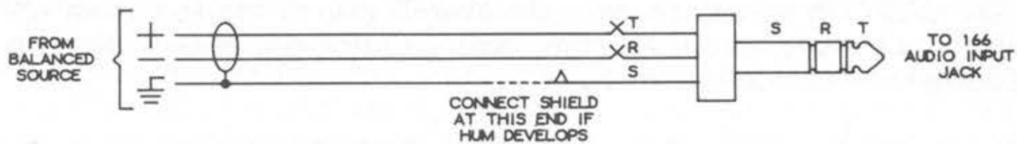
Figure 1: Balanced sources
