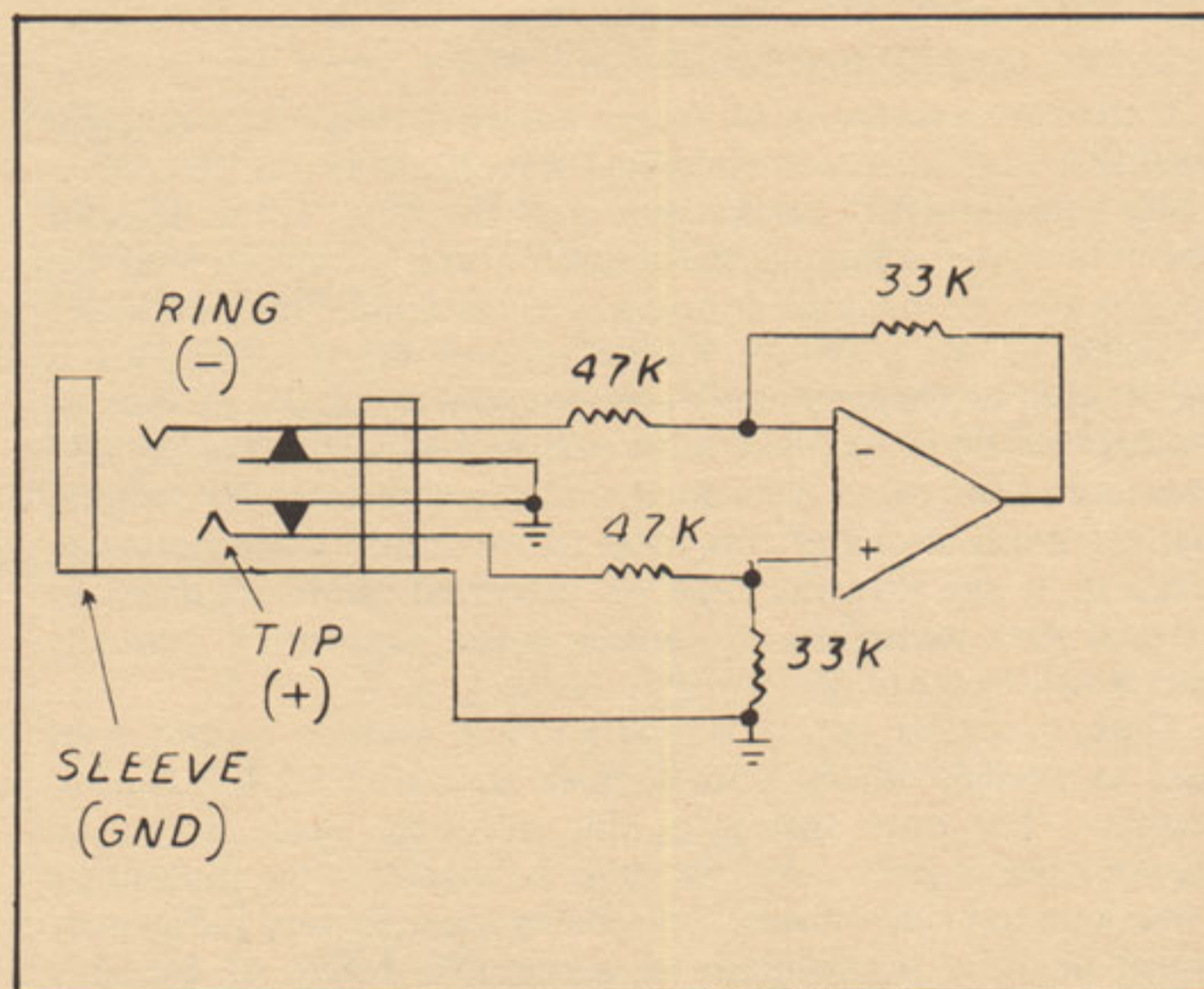
FIGURE 3 INPUT & EXT INPUT CONNECTOR CONFIGURATION (BALANCED)
