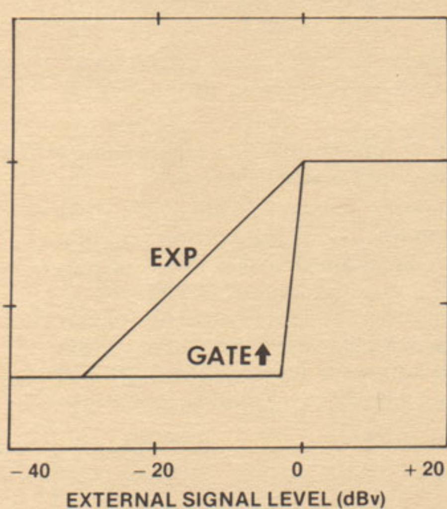
FIGURE 4 SIGNAL GAIN IN RESPONSE TO EXTERNAL CONTROL SIGNAL (EXT DETECT MODE)
