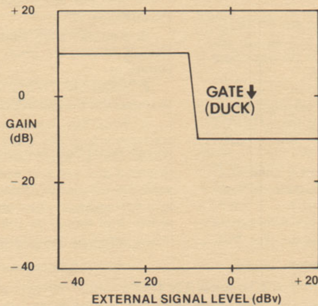
FIGURE 5 SIGNAL GAIN IN RESPONSE TO EXTERNAL CONTROL SIGNAL (EXT DETECT MODE)
