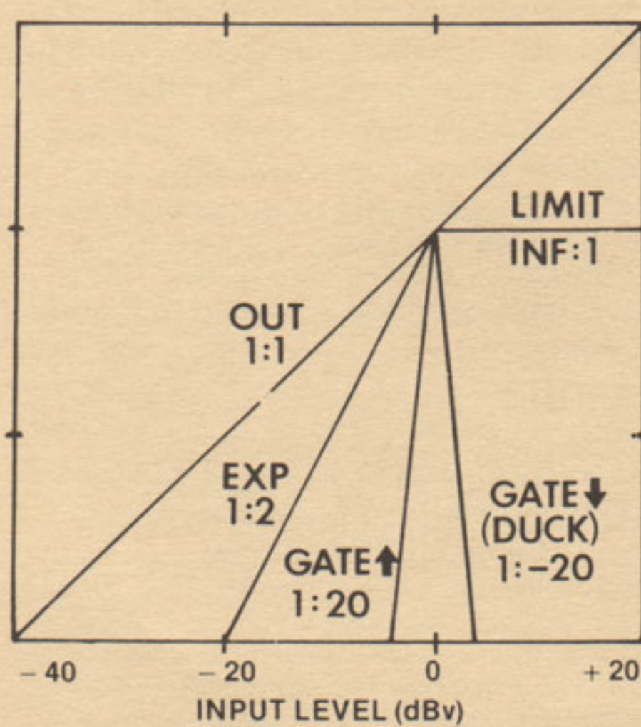
FIGURE 1 BASIC TRANSFER CHARACTERISTICS (INTERNAL DETECT MODE)
