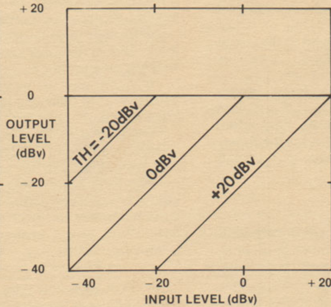
FIGURE 2 EFFECT OF THRESHOLD IN LIMIT MODE
