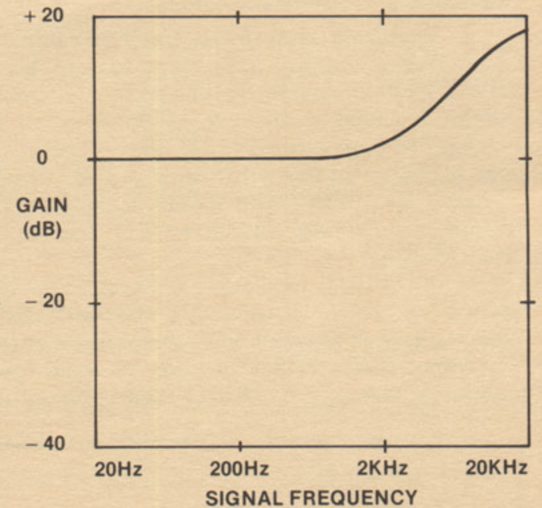
FIGURE 6 SIDE BAND EQUALIZATION APPLIED TO INPUT SIGNAL IN FM-DS MODE
