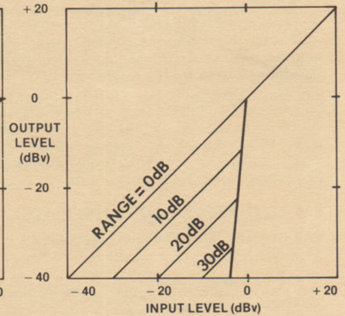
FIGURE 3 EFFECT OF EXP/GATE/DUCK RANGE CONTROL
