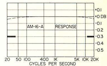
AM-16 AMPLIFIER
