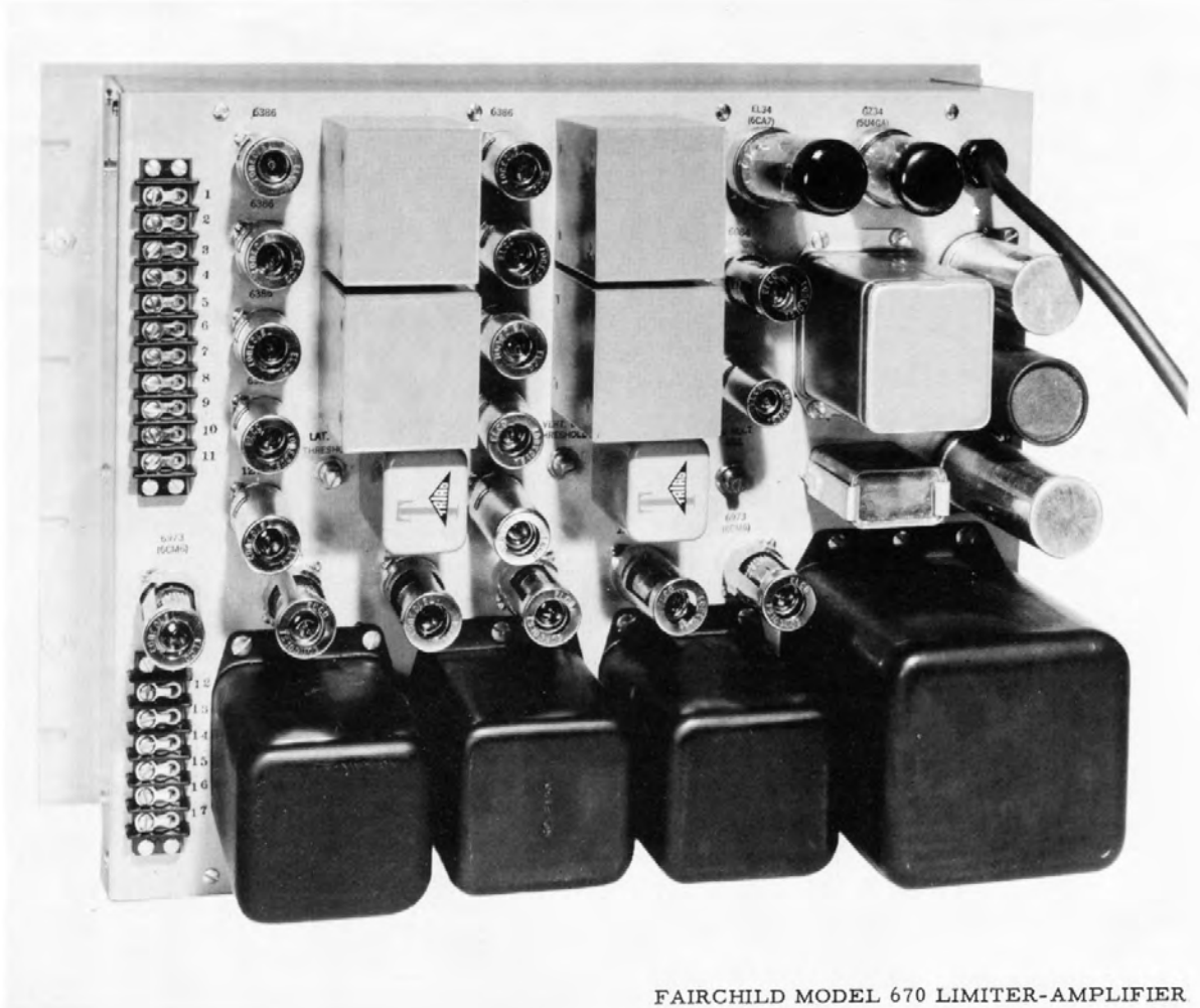
FAIRCHILD MODEL 670 LIMITER-AMPLIFIER TWO-CHANNEL FOR STEREO
