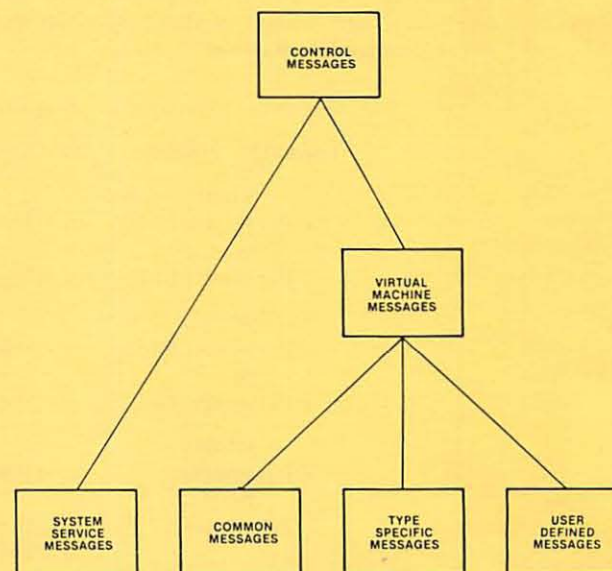
Fig. 1 Message Classification
