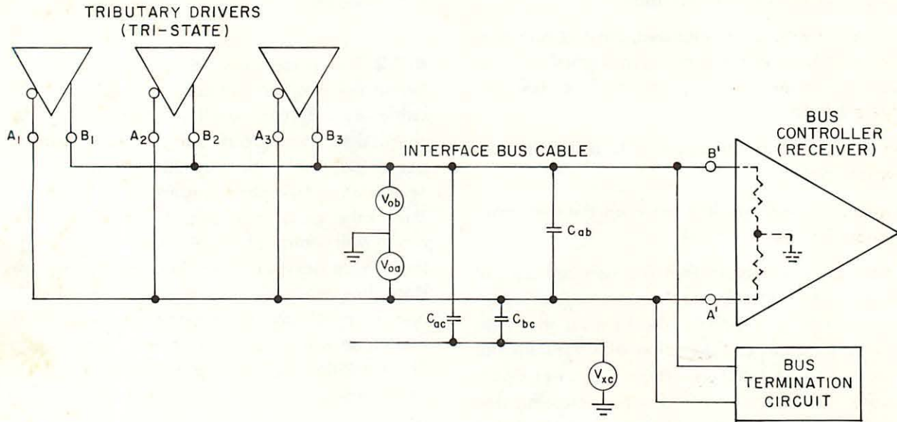
Fig. 8 Cable Model
