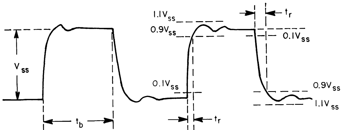
Fig. 3 Generator Output Signal Waveform
