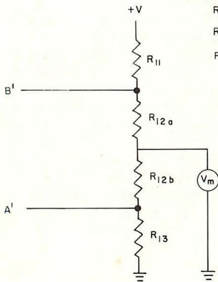
Fig. 9 Terminator Circuit 1
