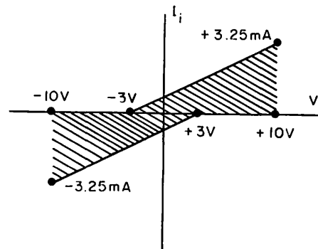
Fig. 4 Receiver Input Current-Voltage Measurement
