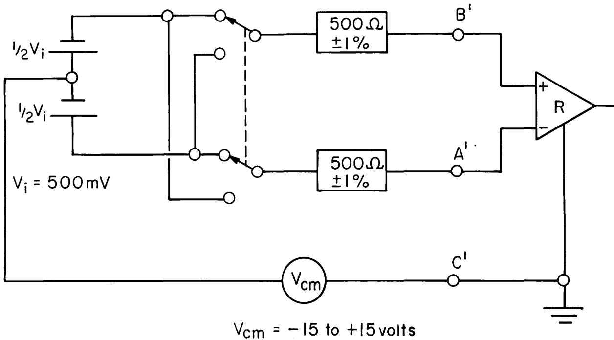
Fig. 6 Receiver Input Balance Measurement
