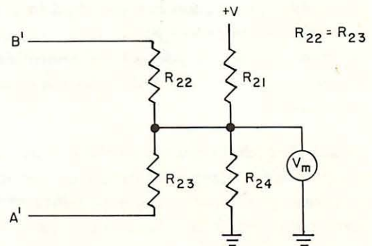
Fig. 10 Terminator Circuit 2
