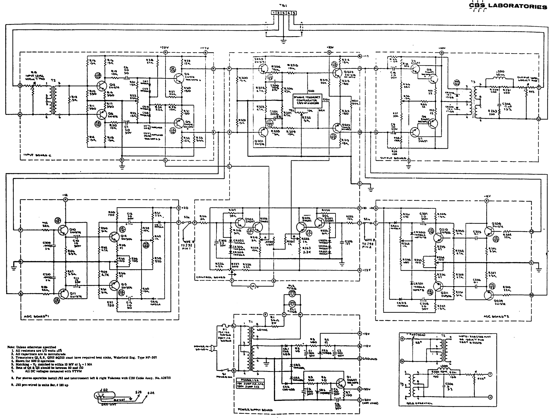
Figure 5-1 FM Volumax Schematic Diagram
