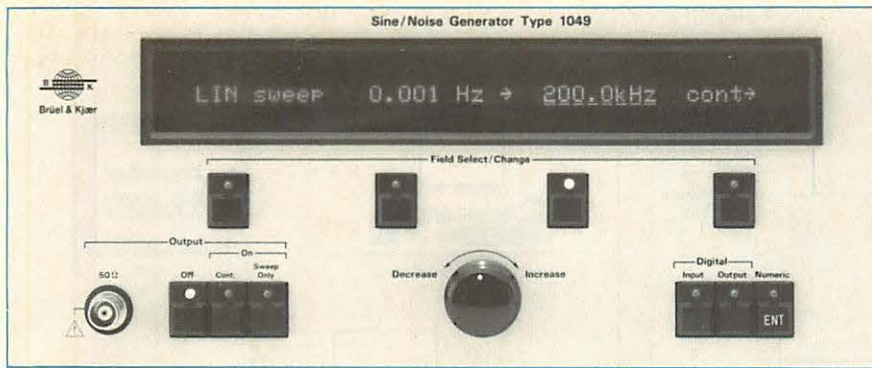
Fig. 5. Vacuum fluorescent line display, plus the field select and speeder controls of the 1049 and 1051
