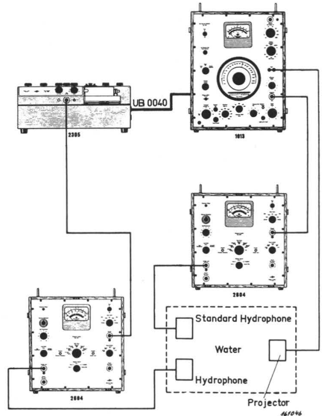
Fig. 8. Recording the frequency response of a hydrophone.
