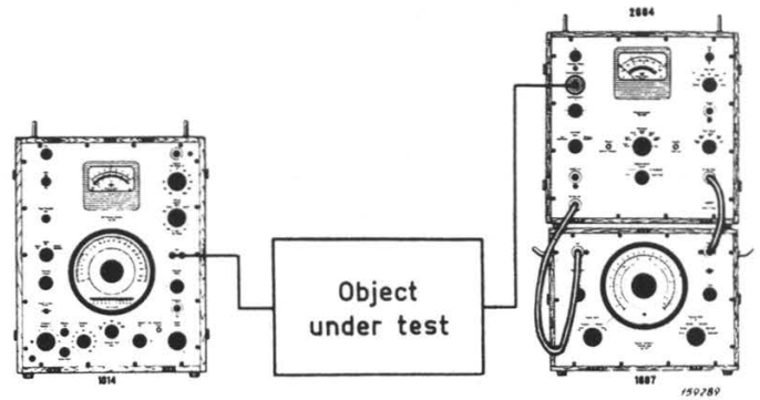
Fig. 7. Measuring arrangement for distortion measurements.
