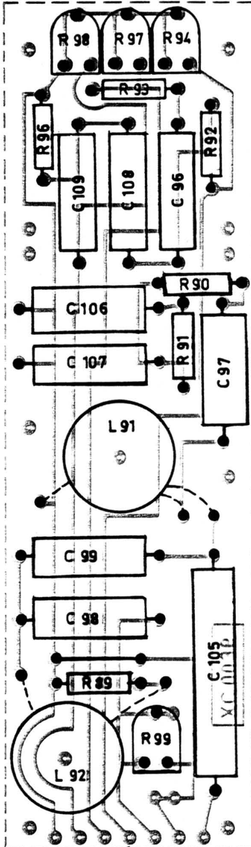
Weighting Network
