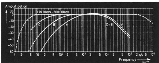
Fig. 2. Typical frequency characteristics of the Microphone Amplifiers. a) Type 2603. b) Type 2604.
