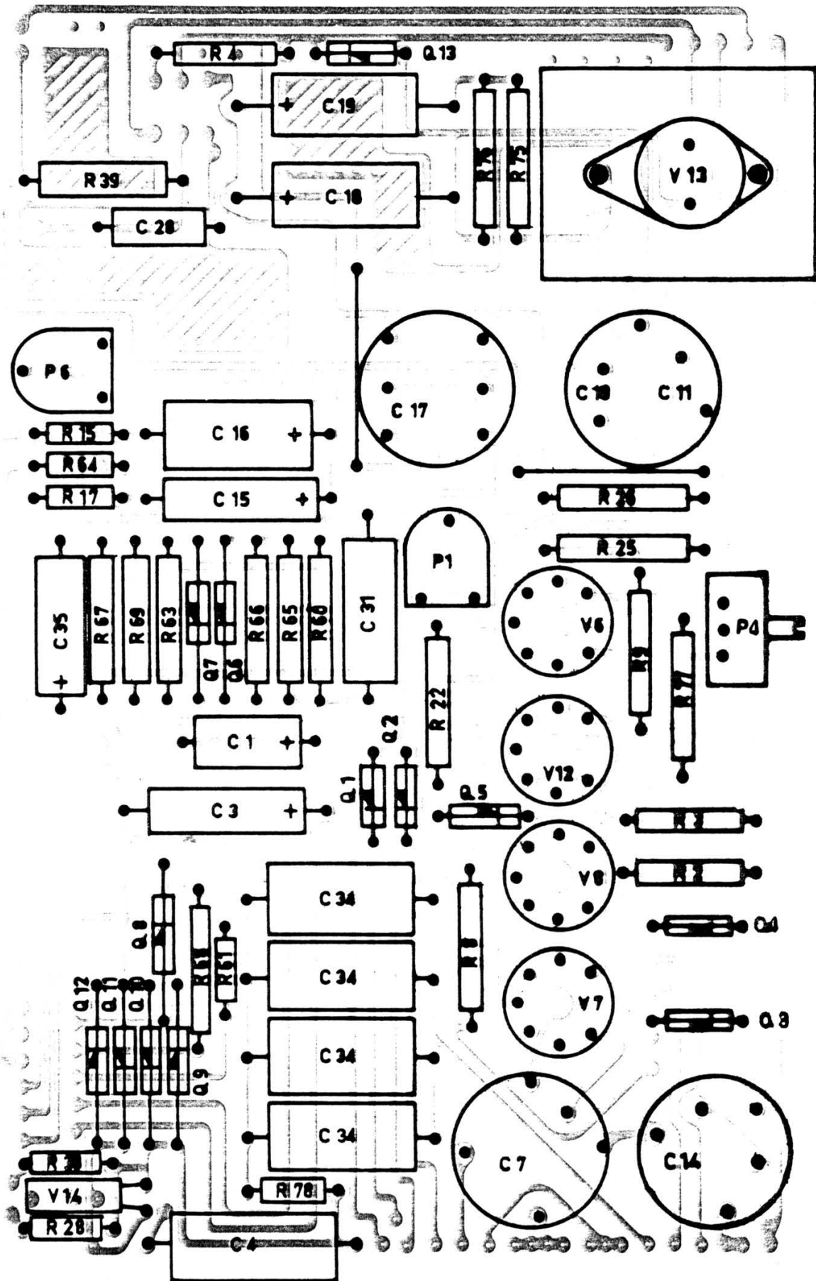
Power Supply
